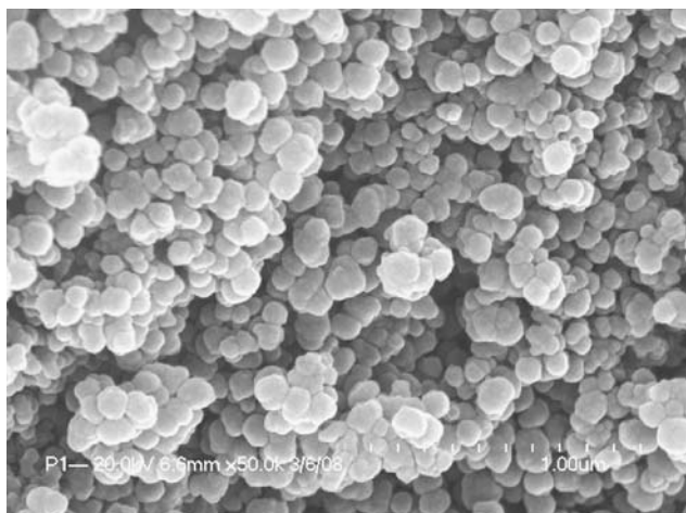
Fig. 1 FE-SEM image of Pd-PEDOT (scale bar 1.00 \mu\text{m} )
