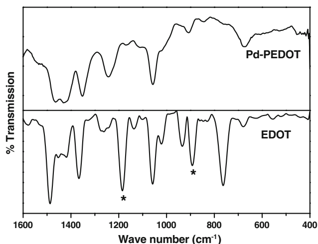
Fig. 4 FT-IR pattern of Pd-PEDOT composite
